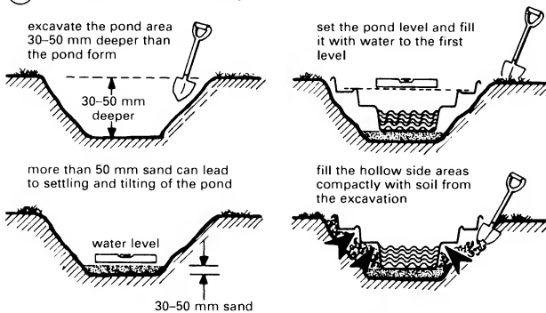
③ Garden pond installation: excavating
